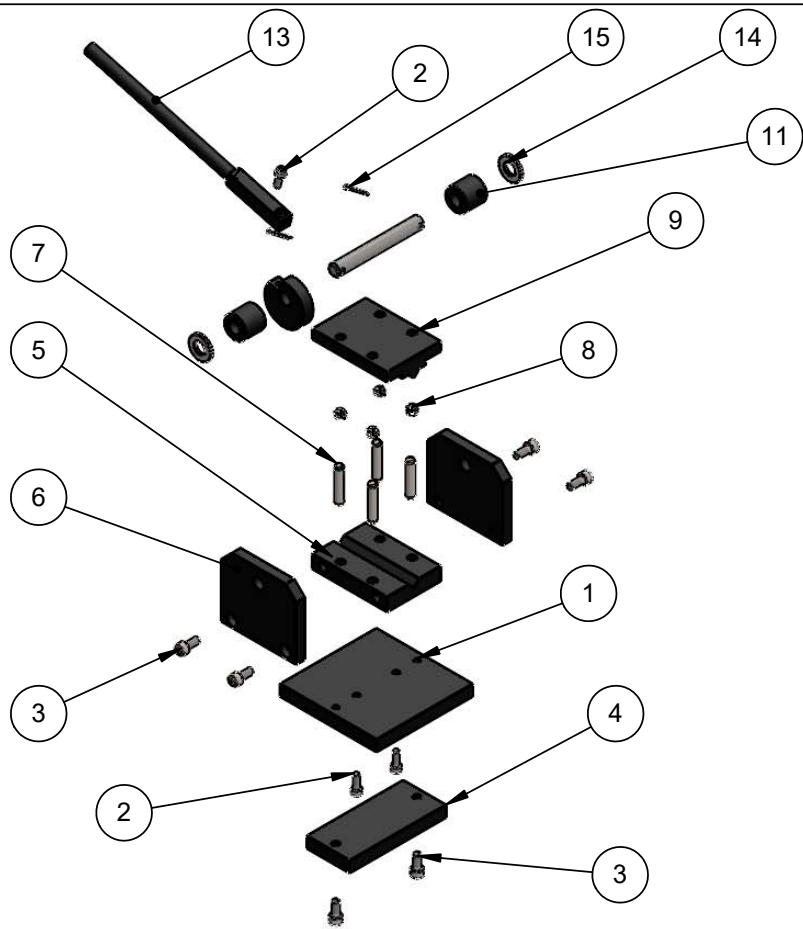
EXPLODED ISOMETRIC VIEW
